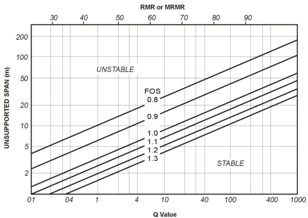
Figure 12 Unsupported span vs Q relationship 12
