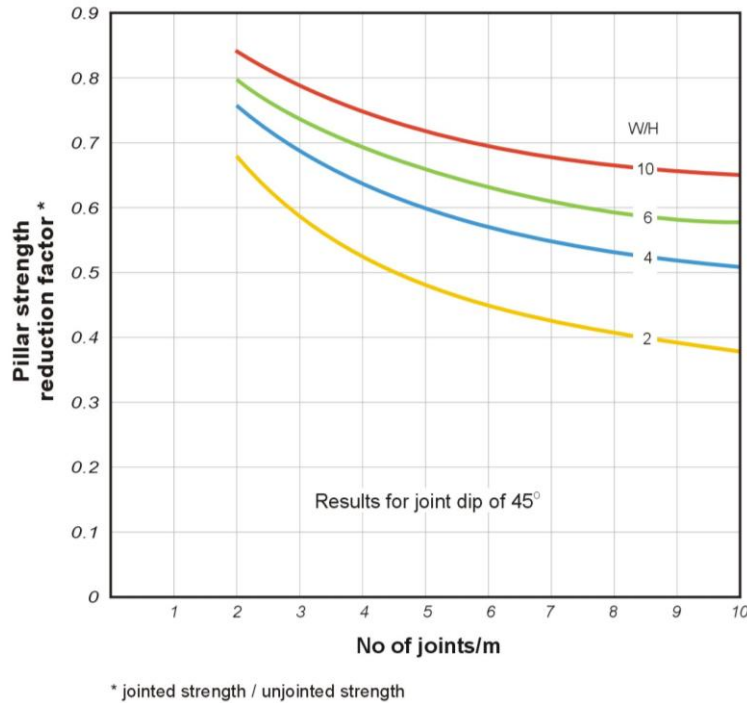
Figure 27 Pillar strength reduction factors for various pillar width to height ratios 7
