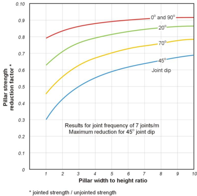
Figure 28 Pillar strength reduction factors for various joint dip angles 7
