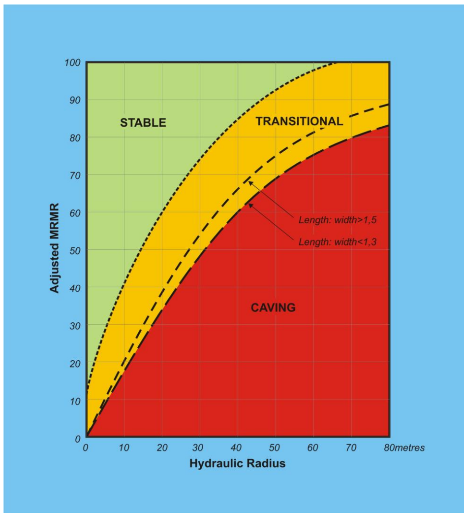
Figure 14 Stability diagram 19
