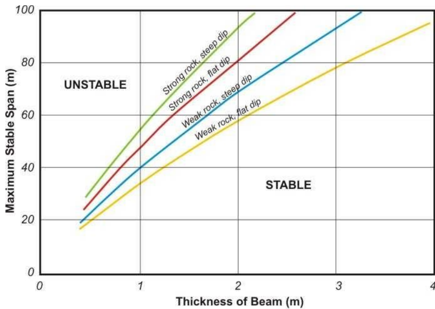
Figure 10 Stability of beams - square excavation (modified 13 )
