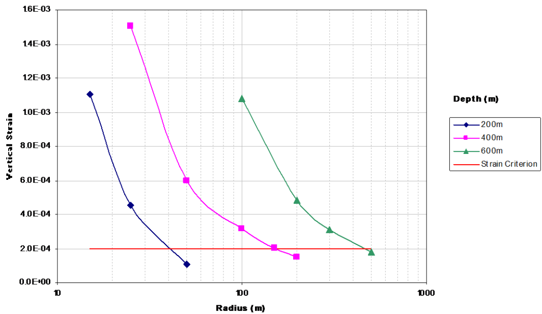
Figure 31 Strain in pillar vs radius - E = 30 GPa
