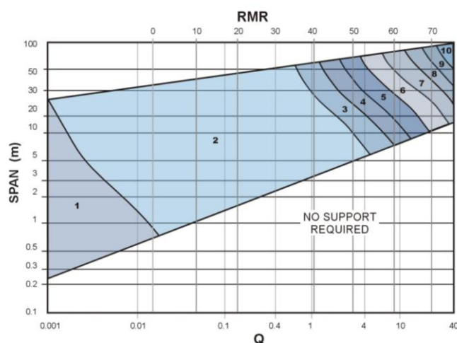
Figure 35 Rockbolt support design chart (modified 1 )
