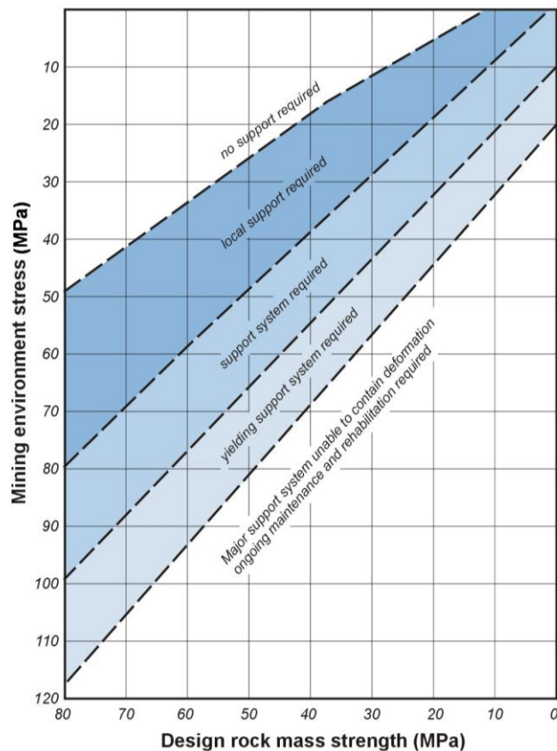
Figure 38 Guideline for drawpoint support 19
