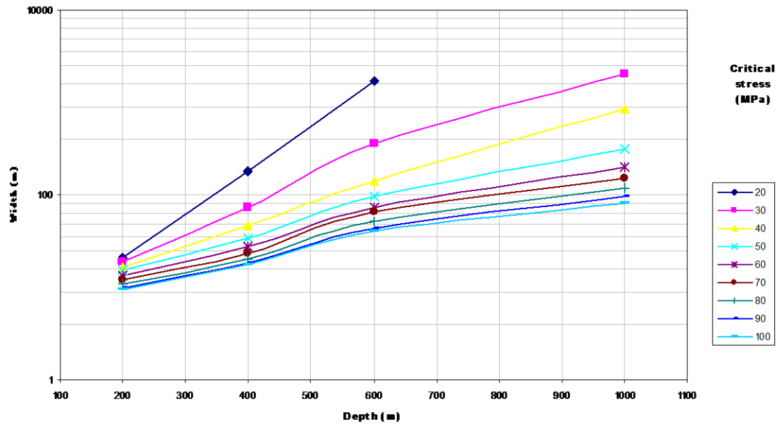
Figure 34 Inclined shaft pillar width vs depth
