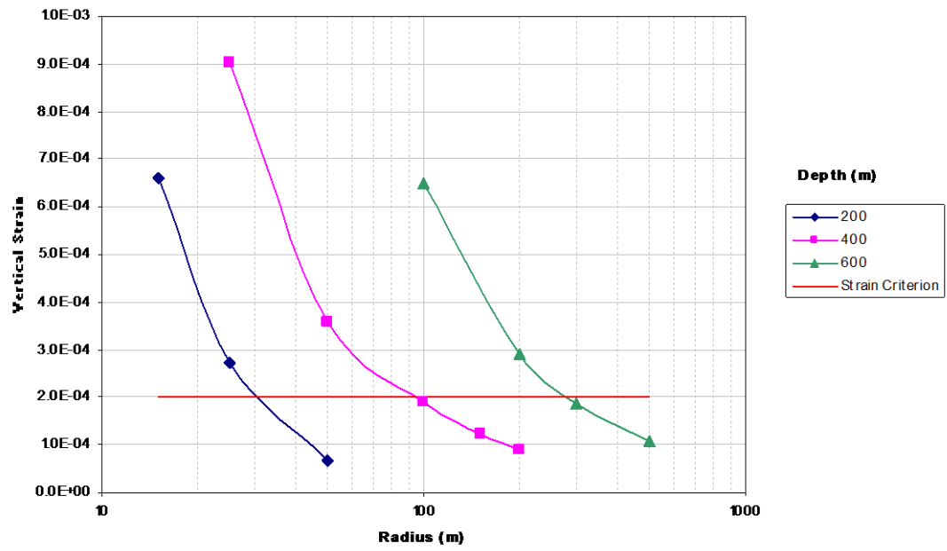
Figure 32 Strain in pillar vs radius - E = 50 GPa
