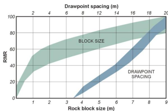
Figure 37 Guideline for fragmentation and drawpoint spacing (modified 19 )
