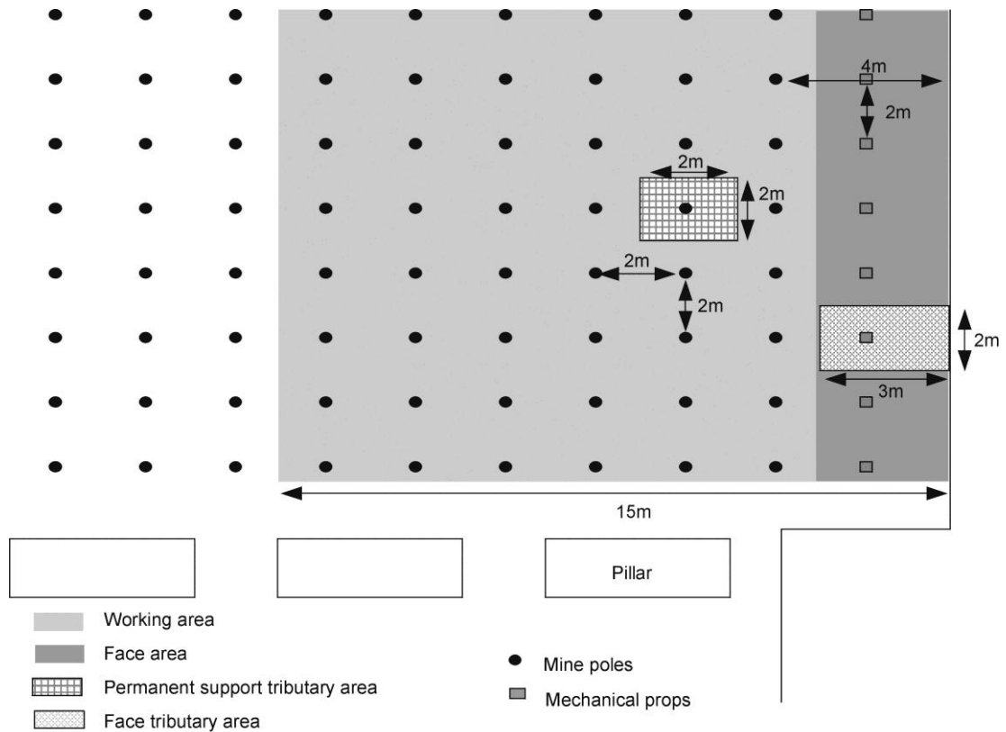
Figure 41 Typical support layout using rockbolts
