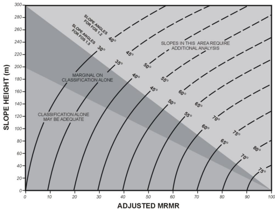
Figure 19 Empirical slope design chart 9
