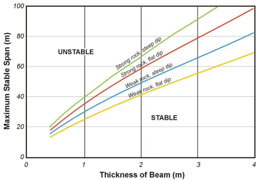
Figure 9 Stability of beams - long excavation (modified 13 )
