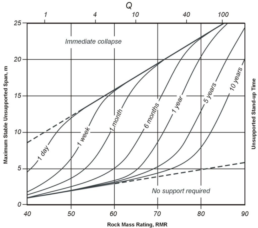
Figure 11 Unsupported span vs RMR relationship 13
