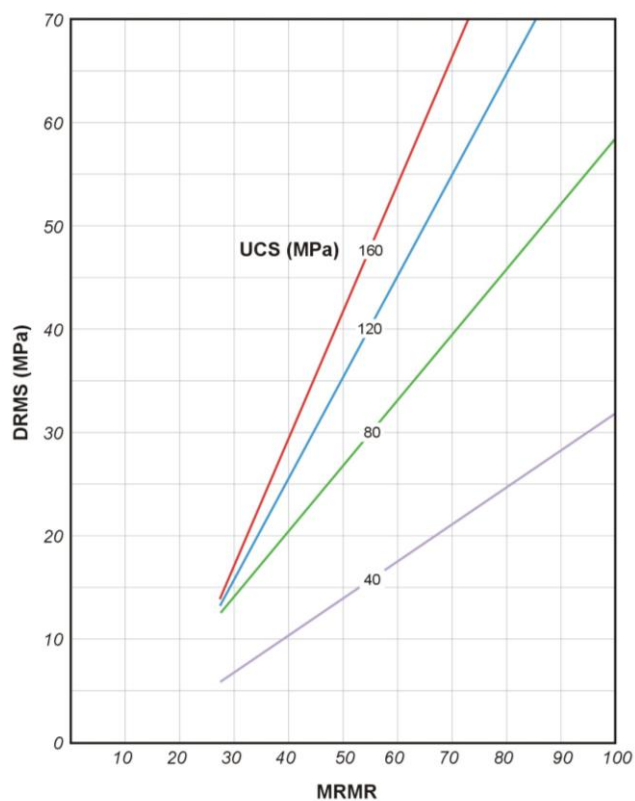
Figure 26 Guideline relationship between DRMS and MRMR
