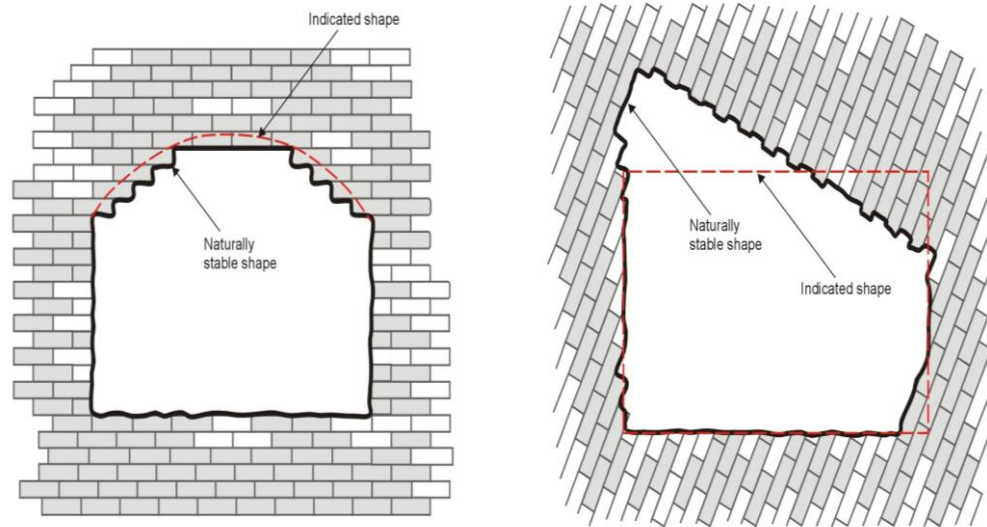
Figure 16 Minimising instability with respect to local geological structure
