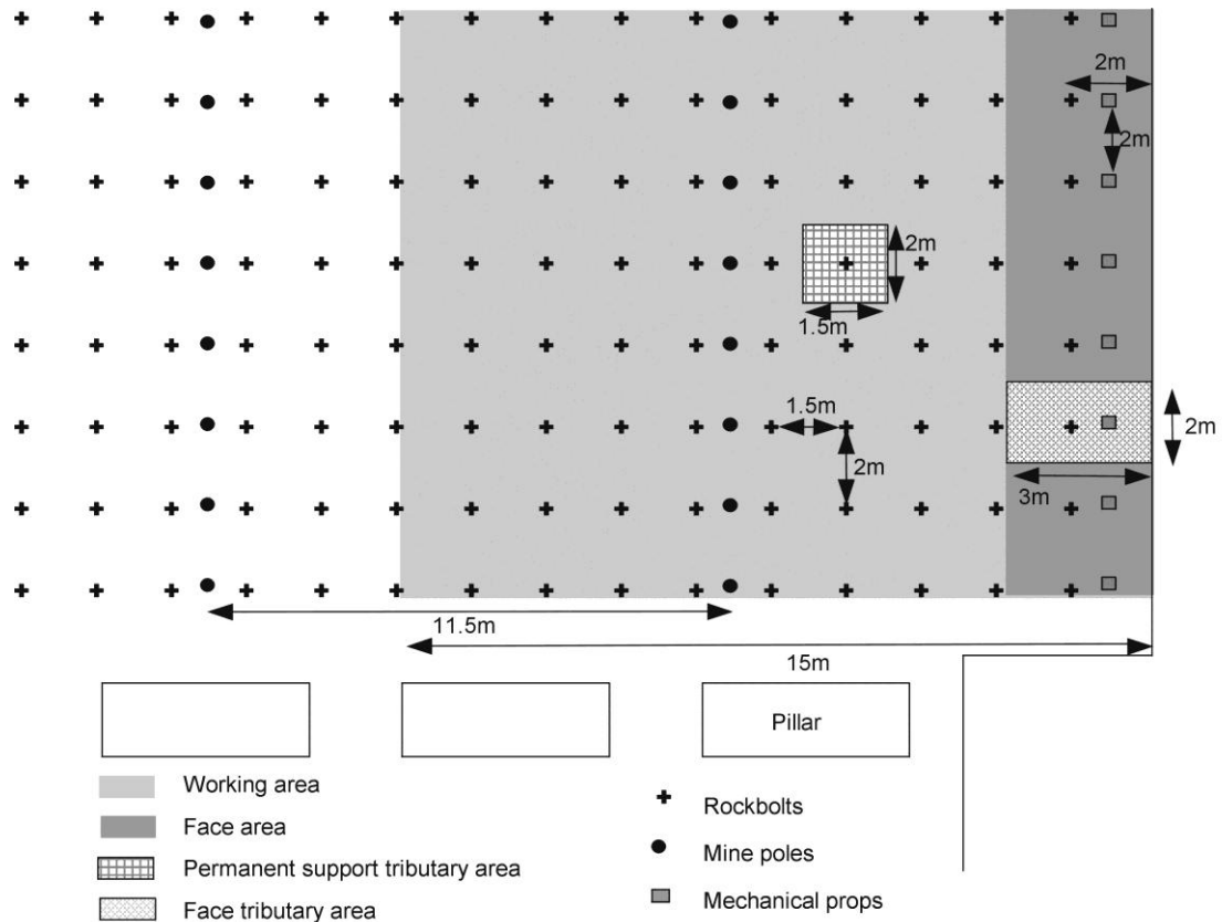
Figure 40 Typical support layout using mine poles
