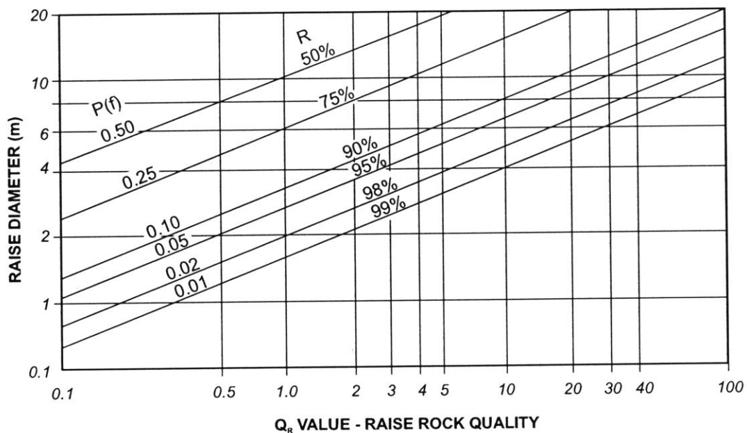
Figure 13 Raisebore reliability chart 21
