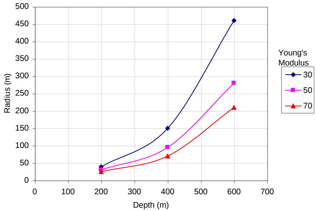
Figure 30 Vertical shaft pillar radius vs depth
