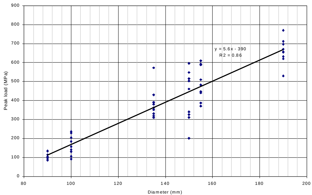
Figure 39 Peak load capacities of mine poles
