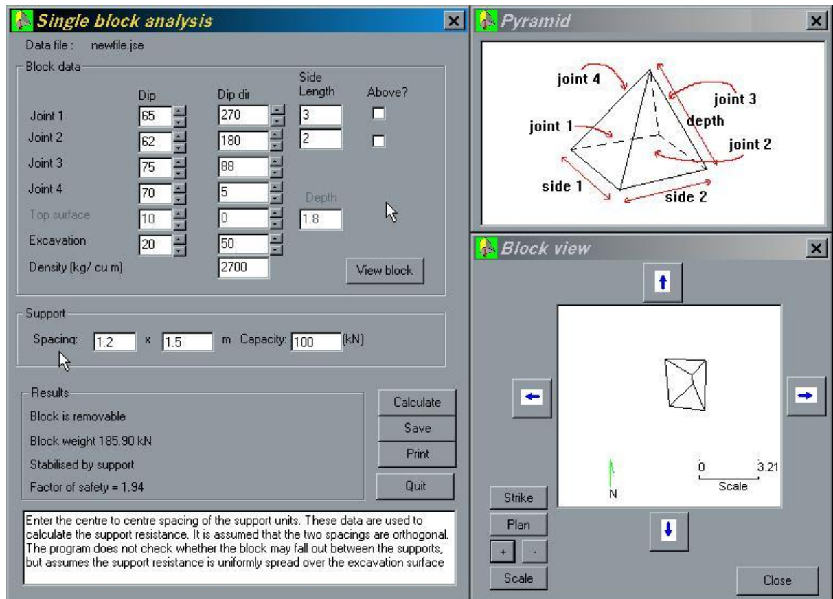
Figure 8 BlockEval windows for input data, output results and block visualization
