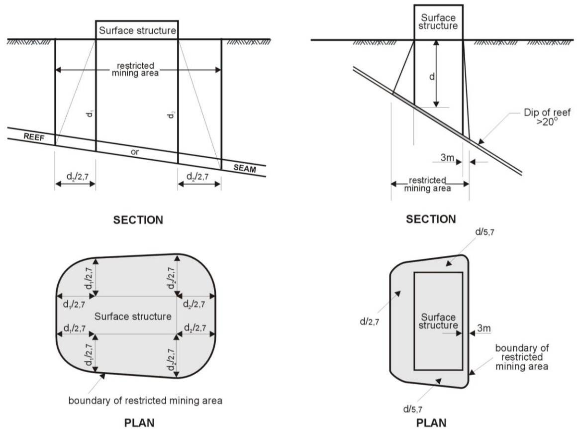
Figure 17 Restrictions on undermining of structures
