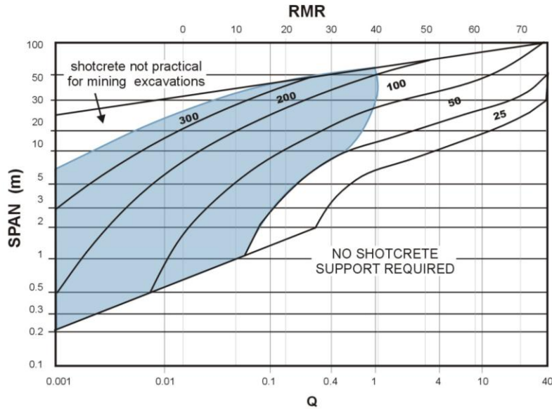
Figure 36 Shotcrete support design chart (modified 1 )
