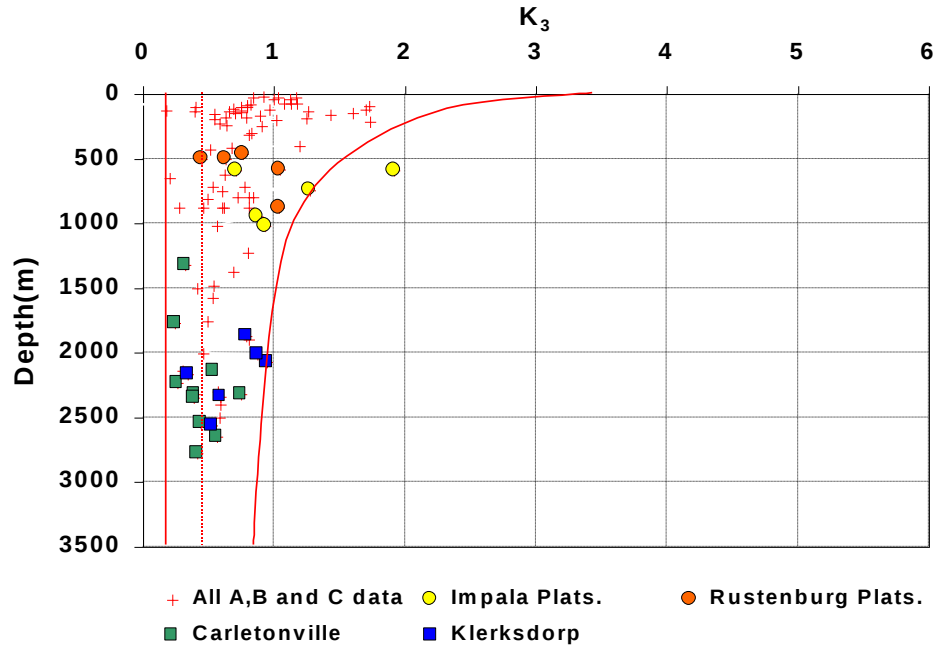
Figure 5 Ratio K_3 of minor horizontal in situ stress to vertical stress 27
