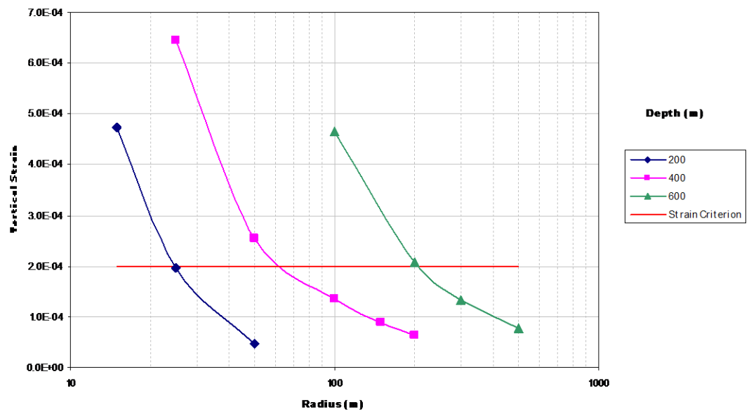
Figure 33 Strain in pillar vs radius - E = 70 GPa
